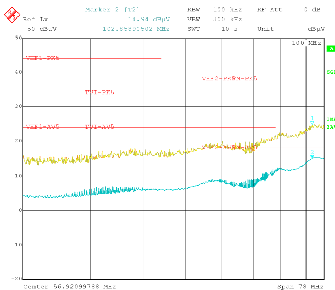
Figure 15. Conducted EMI Measurement with CISPR 25 Class 5 Limit Lines (30 MHz to 110 MHz)
