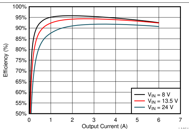
Figure 24. F_{sw} = 400 kHz, 3.3 VOUT, FPWM Mode
