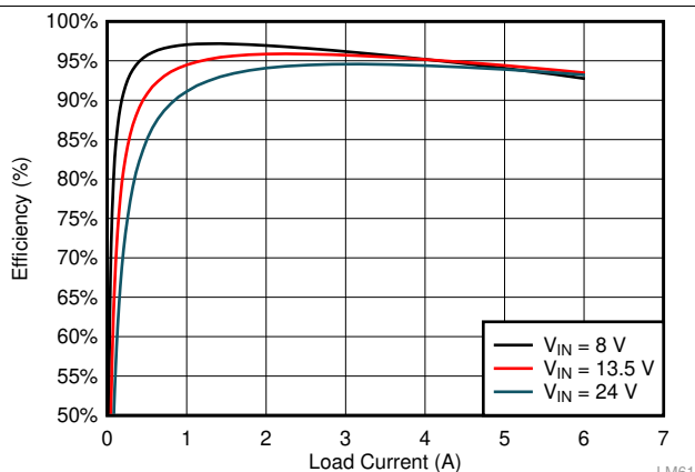
Figure 26. F_{sw} = 2.2 MHz, 5 VOUT, FPWM Mode
