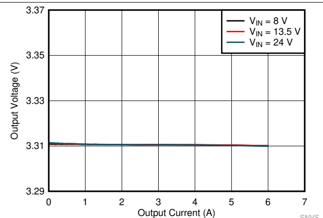
Figure 32. F_{SW} = 400 kHz, 3.3 VOUT, FPWM Mode
