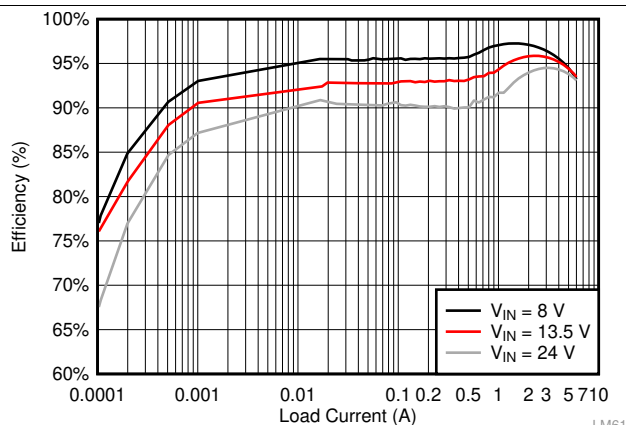
Figure 21. F_{sw} = 400 kHz, 5 VOUT, Auto Mode
