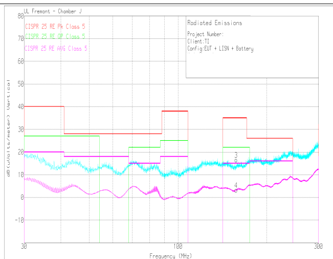
Figure 17. Radiated EMI Measurement with Vertical Bicon Antenna Under CISPR 25 Class 5 Limits
