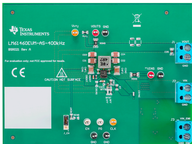
Figure 1. LM61460EVM Front
