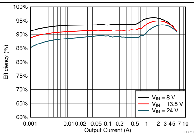
Figure 23. F_{sw} = 400 kHz, 3.3 VOUT, Auto Mode
