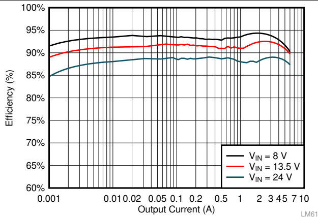
Figure 27. F_{SW} = 2.2 MHz, 3.3 VOUT, Auto Mode
