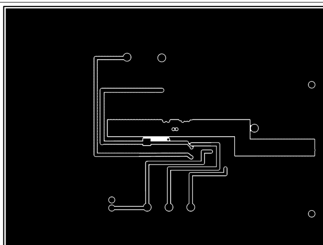
Figure 10. Signal Layer 2 - Routing
