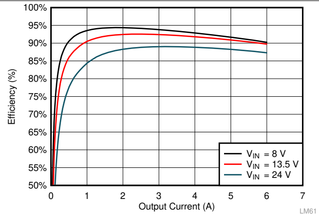
Figure 28. F_{SW} = 2.2 MHz, 3.3 VOUT, FPWM Mode
