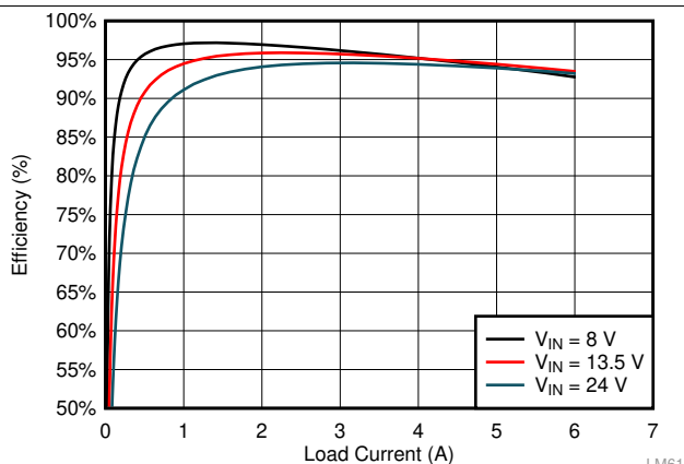
Figure 22. F_{sw} = 400 kHz, 5 VOUT, FPWM Mode
