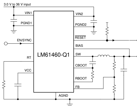
Figure 4. LM61460-Q1 Schematic
