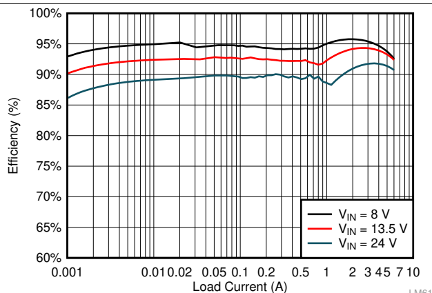
Figure 25. F_{sw} = 2.2 MHz, 5 VOUT, Auto Mode
