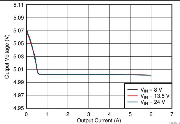
Figure 29. F_{SW} = 400 kHz, 5 VOUT, Auto Mode
