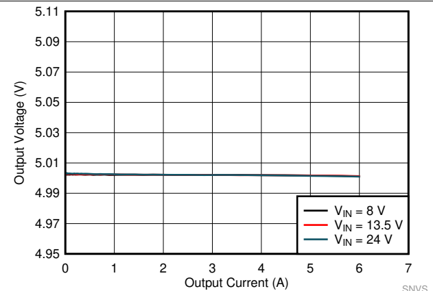
Figure 30. F_{SW} = 400 kHz, 5 VOUT, FPWM Mode
