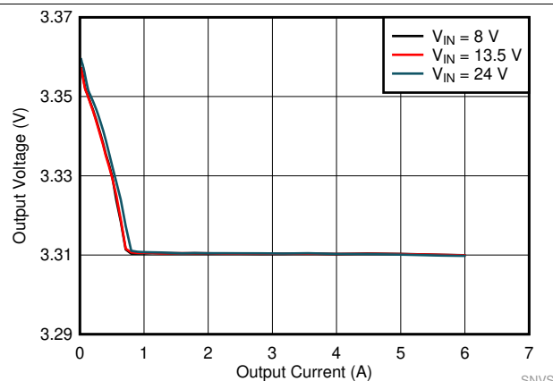
Figure 31. F_{SW} = 400 kHz, 3.3 VOUT, Auto Mode
