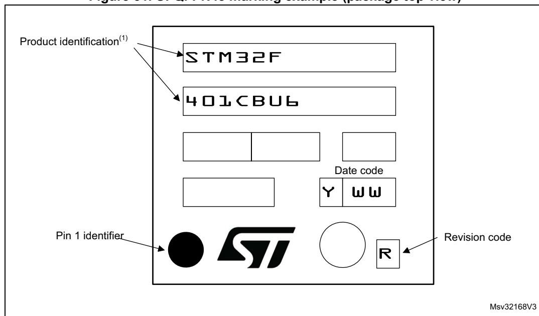
Figure 51. UFQFPN48 marking example (package top view)
