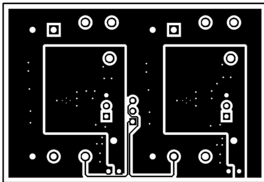
Figure 7. Bottom Layer
