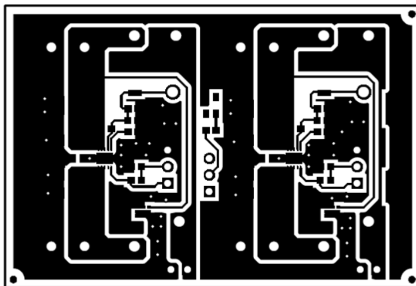
Figure 6. Top Layer
