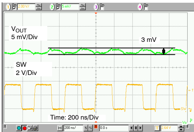
Figure 13. Output Ripple Voltage ( V_{IN} = 3.6 \text{ V} , V_{OUT} = 1.8 \text{ V} , I_{OUT} = 1 \text{ A} , L = 1.0 \mu\text{H} , C_{OUT} = 10 \mu\text{F} )
