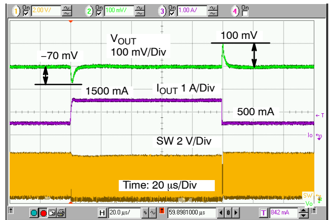
Figure 14. Load Transient Response ( V_{IN} = 3.6 \text{ V} , V_{OUT} = 1.8 \text{ V} , I_{OUT} = 500 \text{ mA} to 1500 \text{ mA} , L = 1.0 \mu\text{H} , C_{OUT} = 10 \mu\text{F} )
