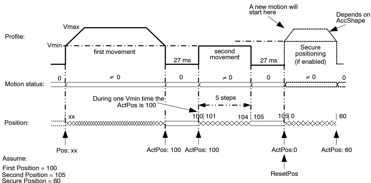
Figure 8. Dual Positioning
