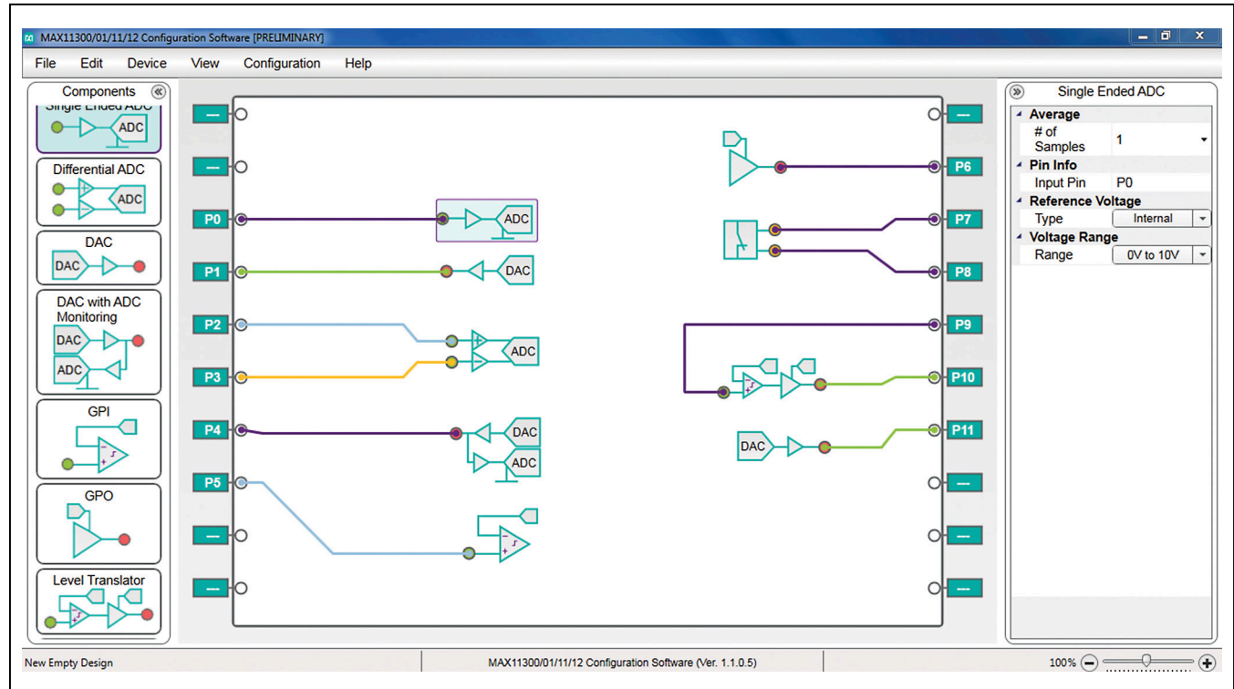
Figure 13. Example of GUI to Develop Configuration File
