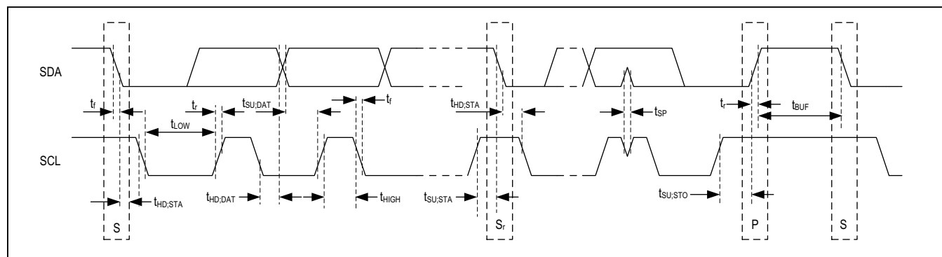
Figure 1. I 2 C Timing
