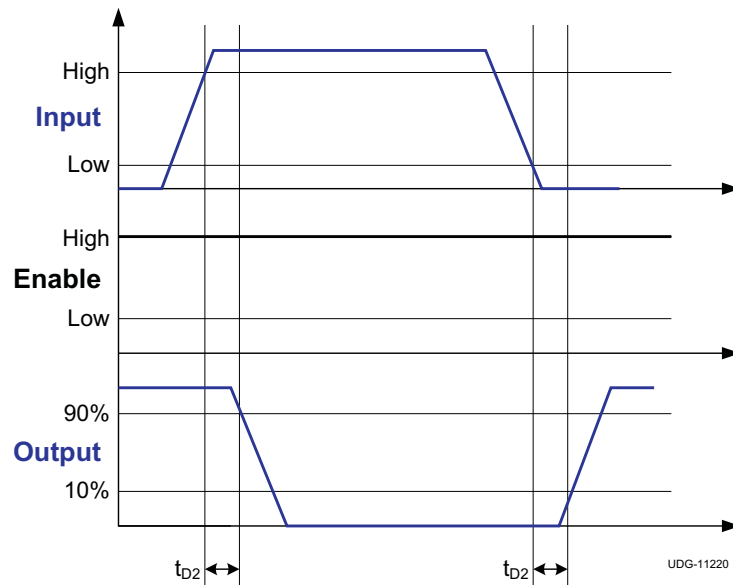
Figure 2. Inverting Configuration
