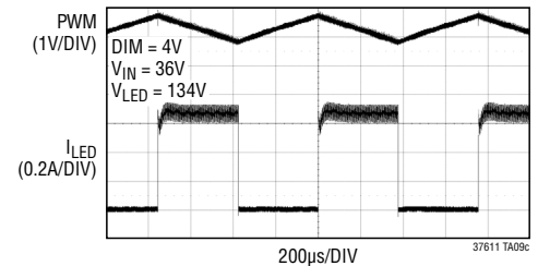
Dimming Waveform
