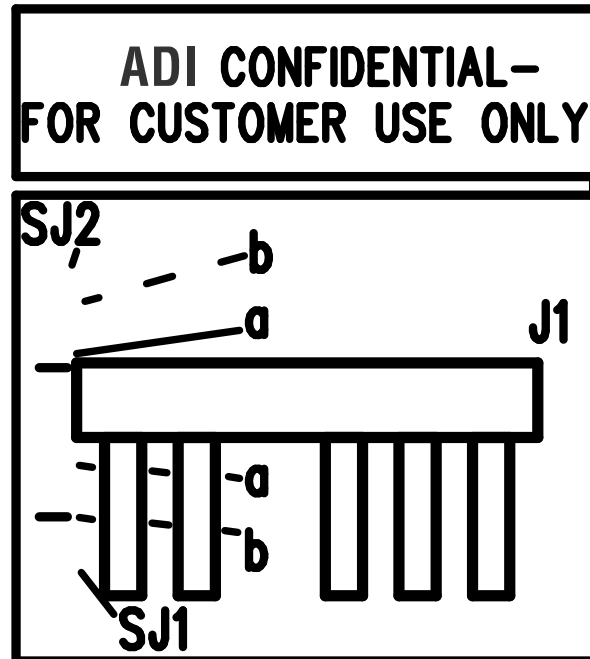
Top Silkscreen
