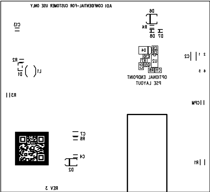
Silkscreen Bottom
