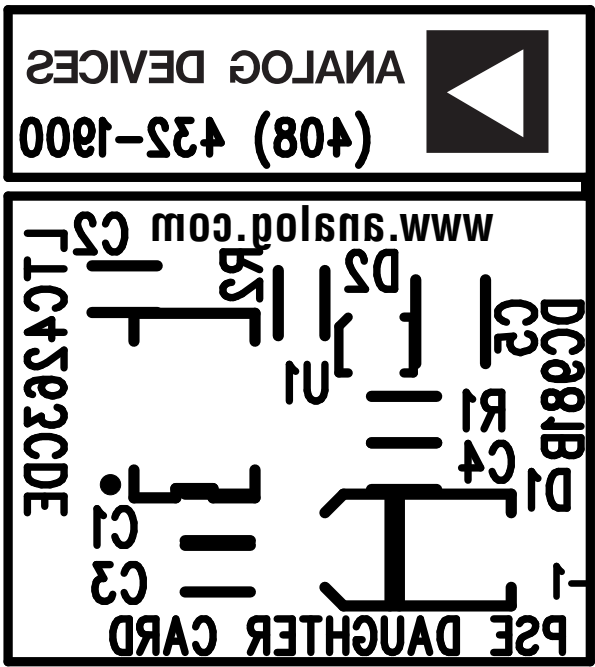
Bottom Silkscreen
