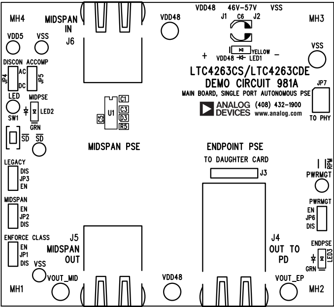
Top Silkscreen
