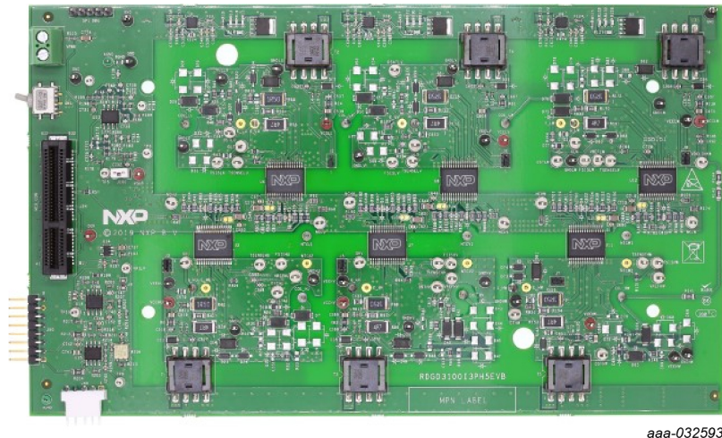
Figure 1. RDGD3100I3PH5EVB
