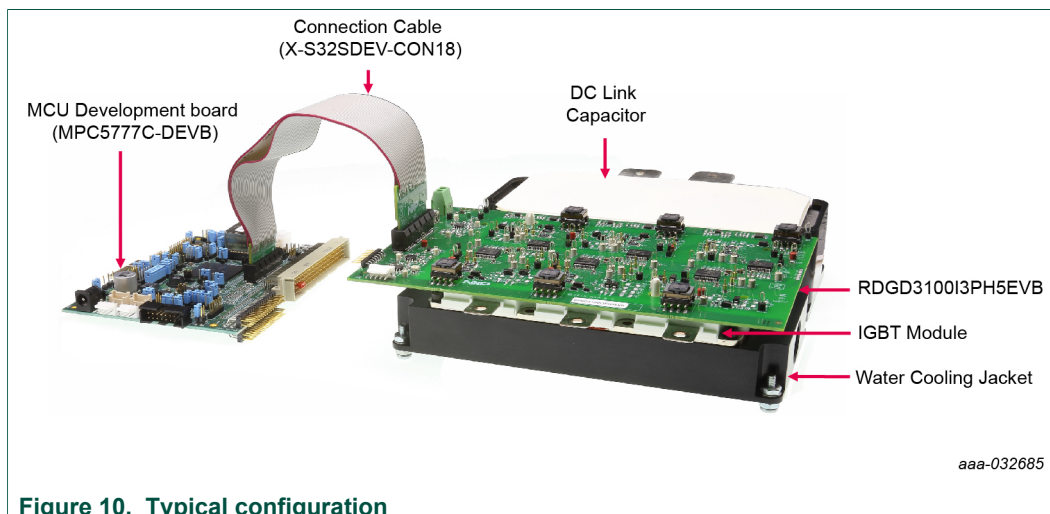
Figure 10. Typical configuration
