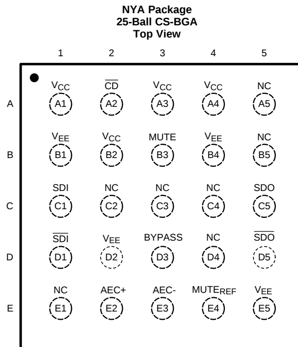
Pin Functions – NYA Package
