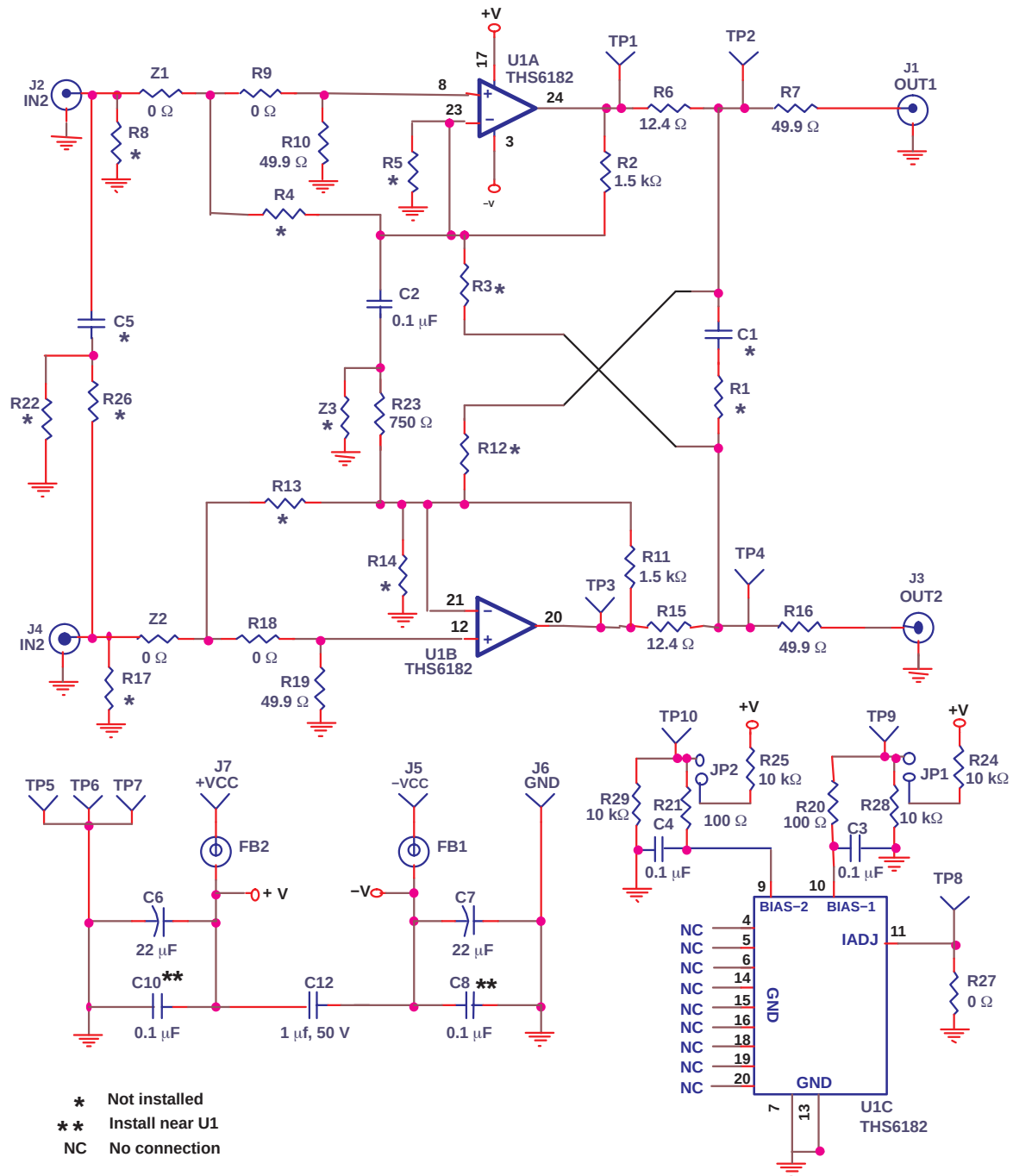
Figure 1–1. Full Schematic of the Populated Circuit on the THS6182RHFEM (Default Configuration)
