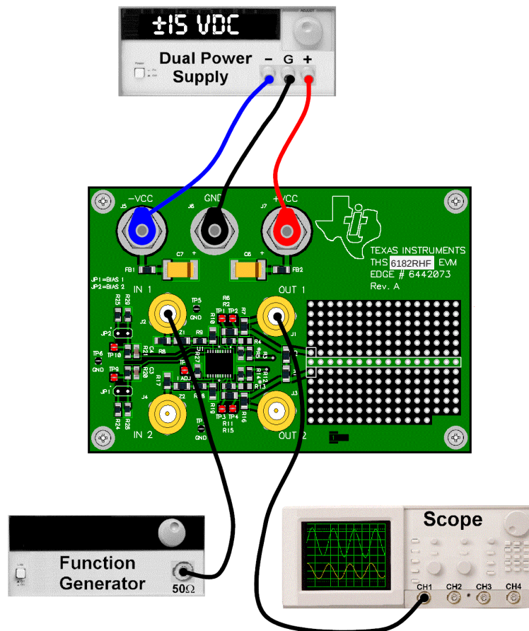
Figure 2–1. Interconnection Diagram
