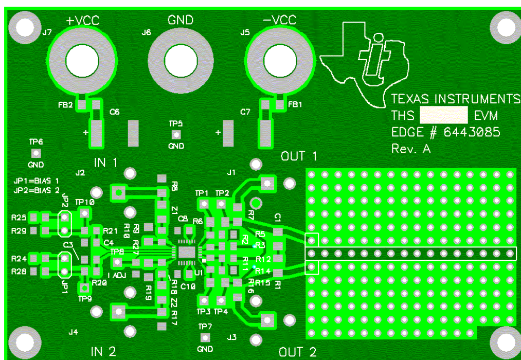
Figure 4–1. Top Layer 1 (Signals for THS6182RHFEVM)
