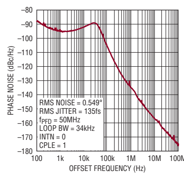
System Phase Noise, f_{RF} = 11.260\text{GHz}
