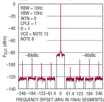
Spurious Response
