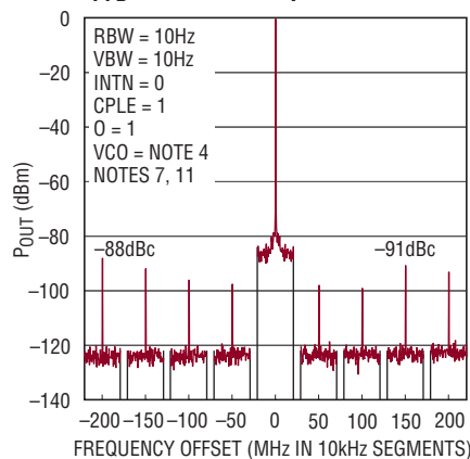
Spurious Response
