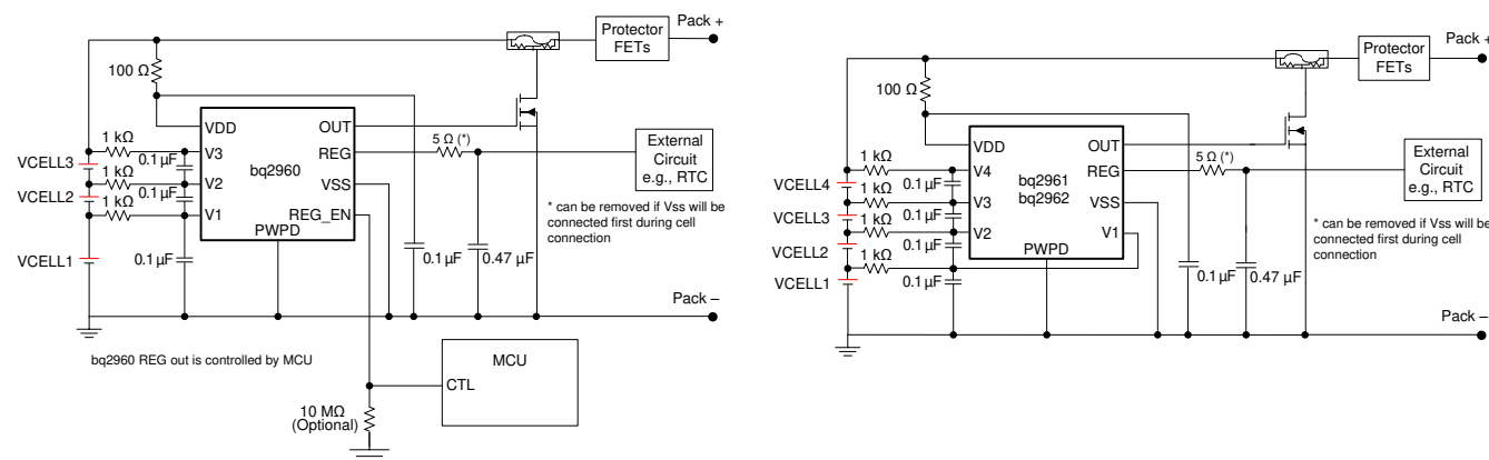
Figure 16. Application Schematic
