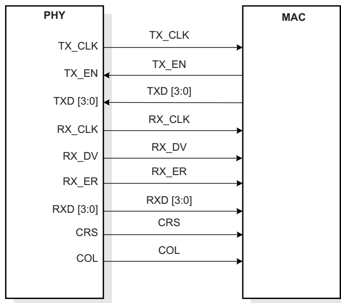
Figure 6-1. MII Signaling
