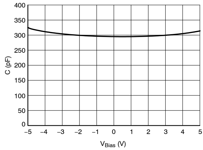
Figure 7. CV Characteristics
