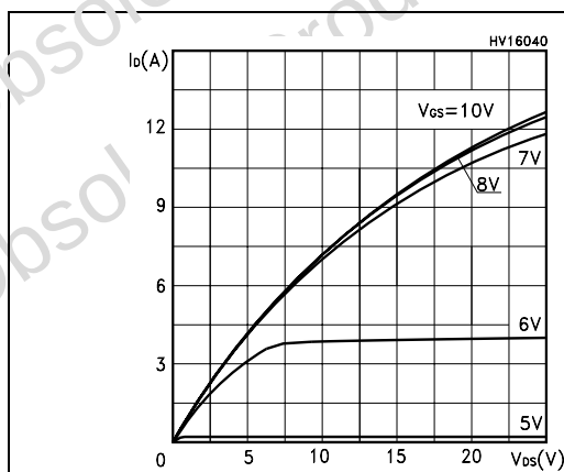
Figure 5. Output characteristics
