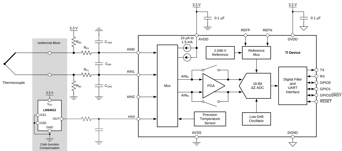
Figure 76. Thermocouple Measurement
