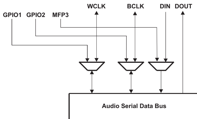
Figure 13. Alternate Audio Bus Multiplexing Function
