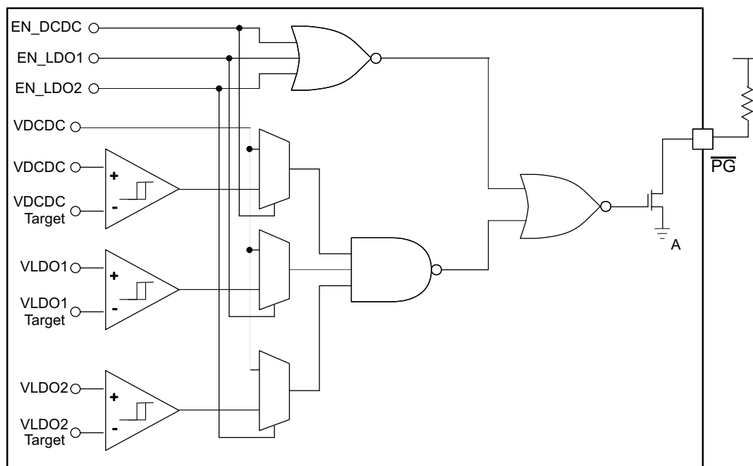
Figure 22. Power-Good Functionality
