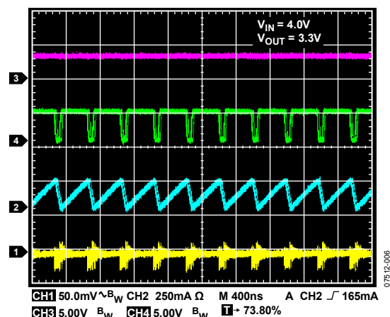
Figure 6. Buck Operation, V_{IN} = 4.0\text{ V} , V_{OUT} = 3.3\text{ V} , I_{LOAD} = 500\text{ mA} , PWM
