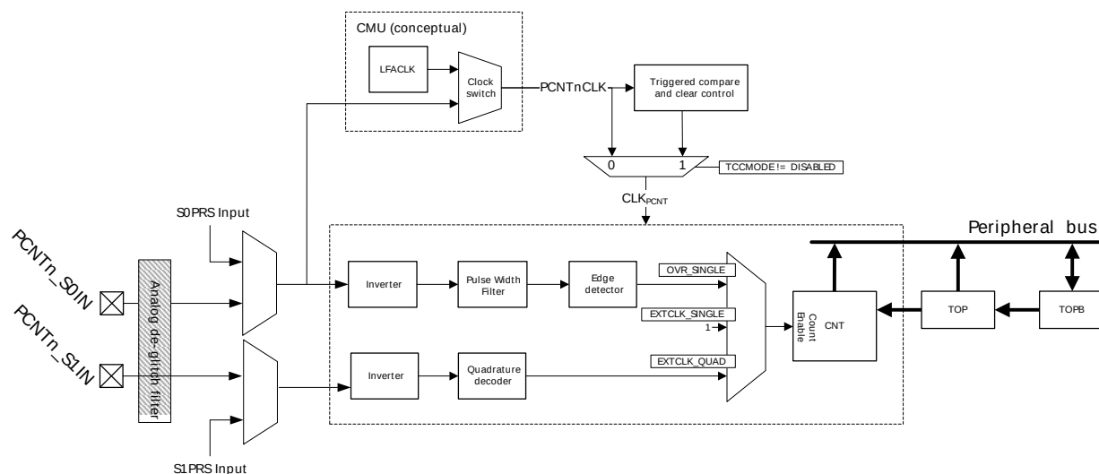
Figure 19.1. PCNT Overview
