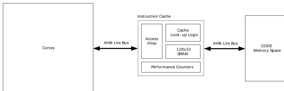
Figure 7.1. Instruction Cache
