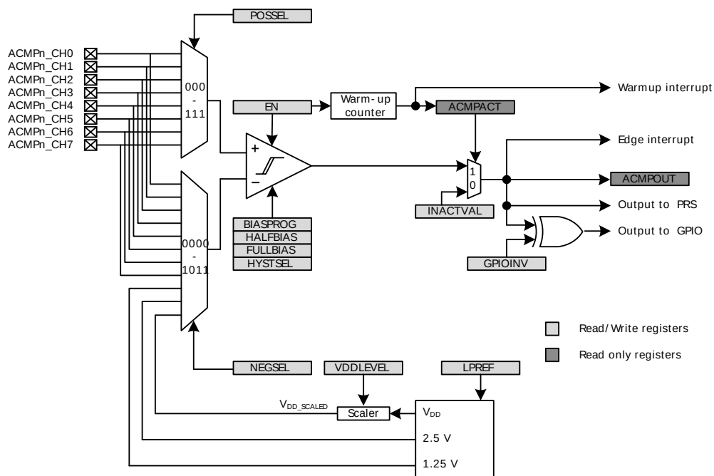
Figure 20.1. ACMP Overview
