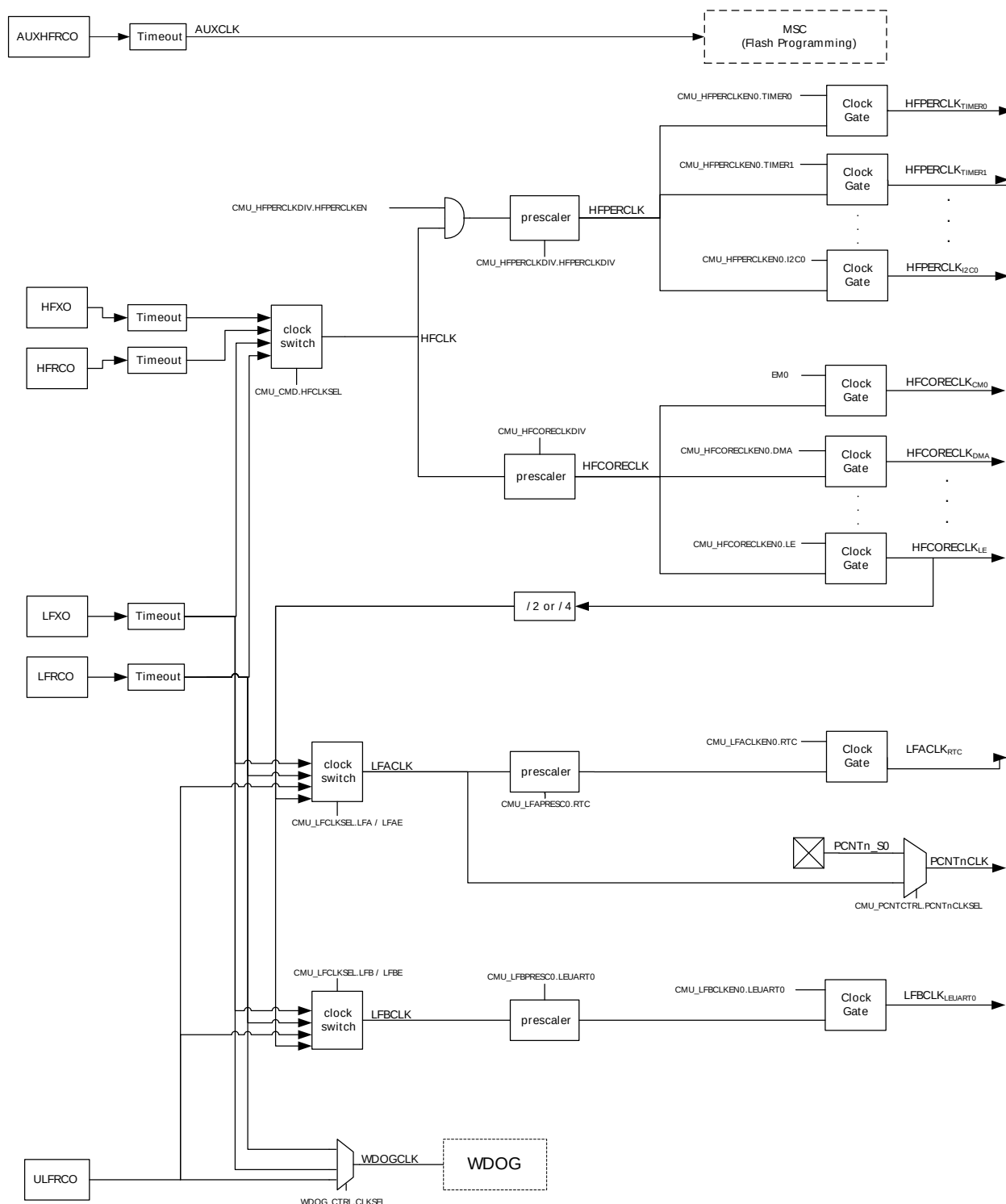
Figure 11.1. CMU Overview
