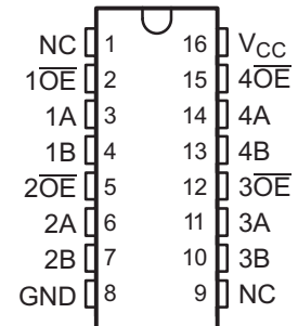
DBQ Package 16-Pin SSOP Top View
