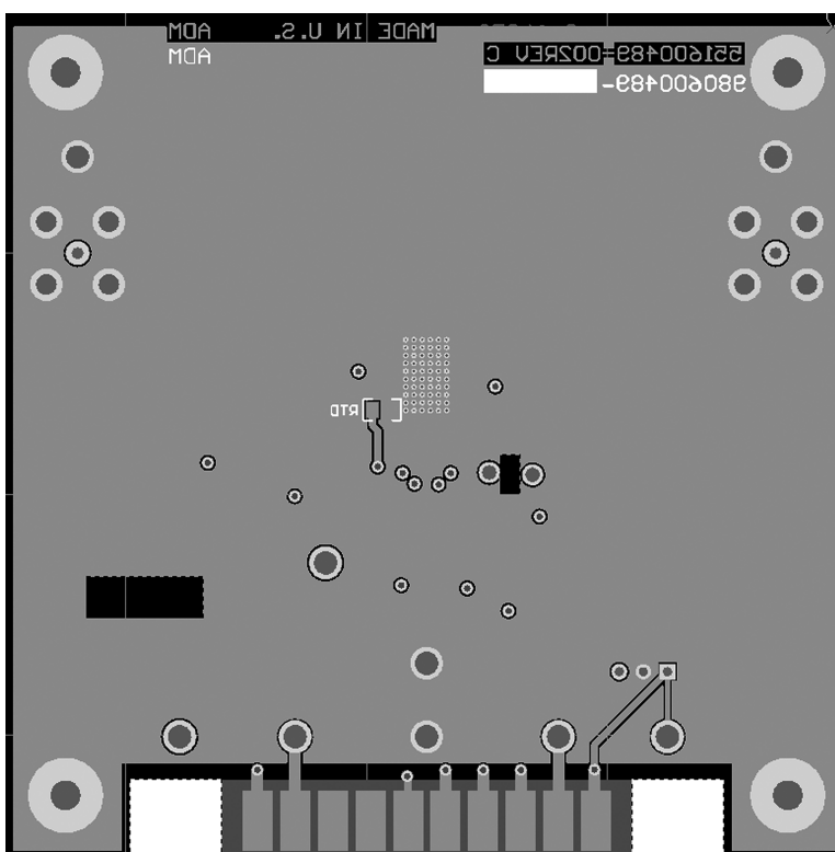
Figure 6. Bottom Layer (Ground) Heat Sinking Layer
