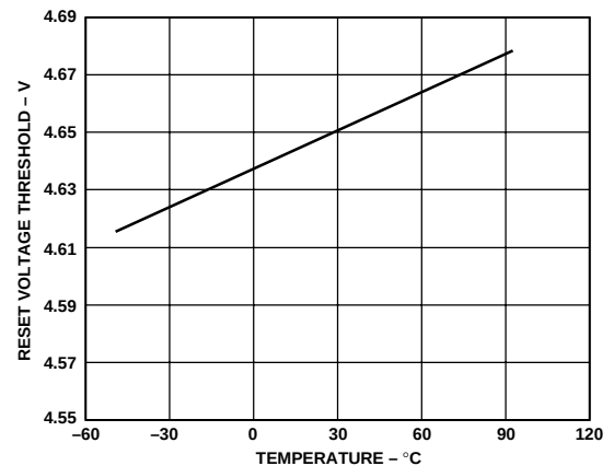
Figure 3. \overline{RESET} Voltage Threshold vs. Temperature
