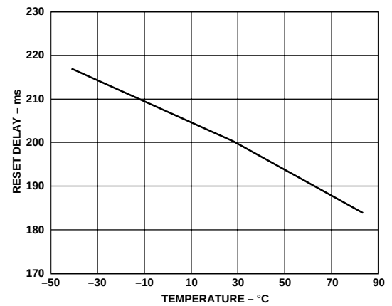
Figure 2. \overline{RESET} Timeout Delay vs. Temperature
