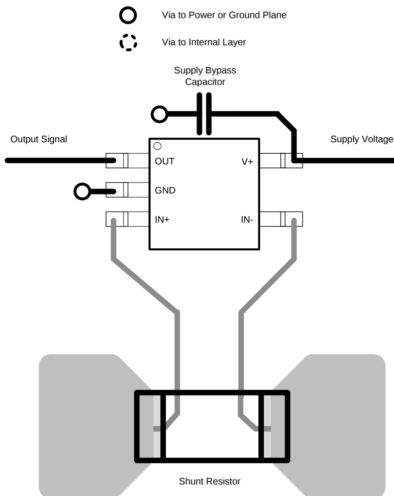
Figure 31. Recommended Layout
