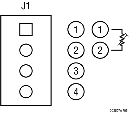
Figure 5. 2-Wire RTD Connection
