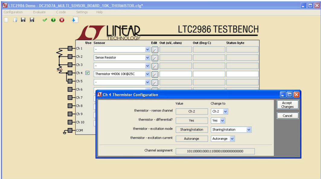
Figure 12. Thermistor Configuration
