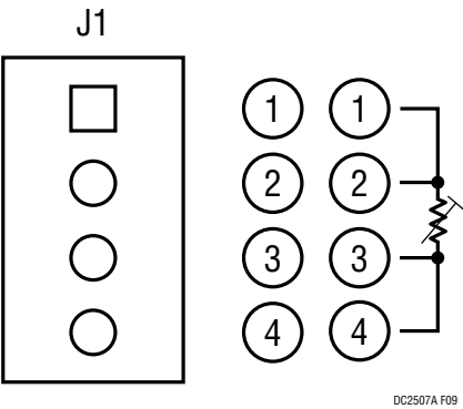
Figure 9. 4-Wire RTD Connection
