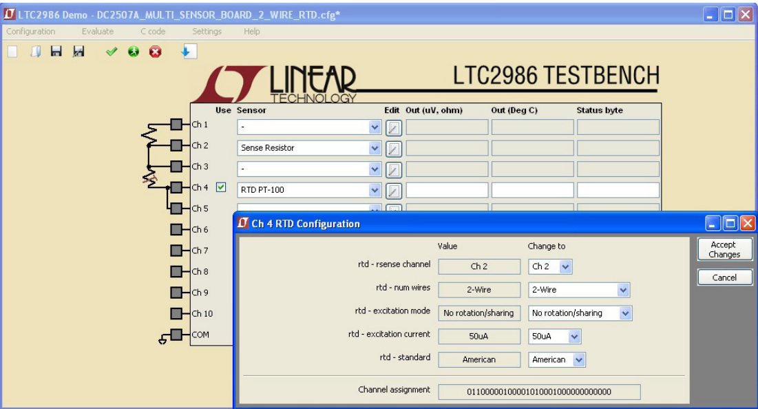
Figure 6. 2-Wire RTD Configuration
