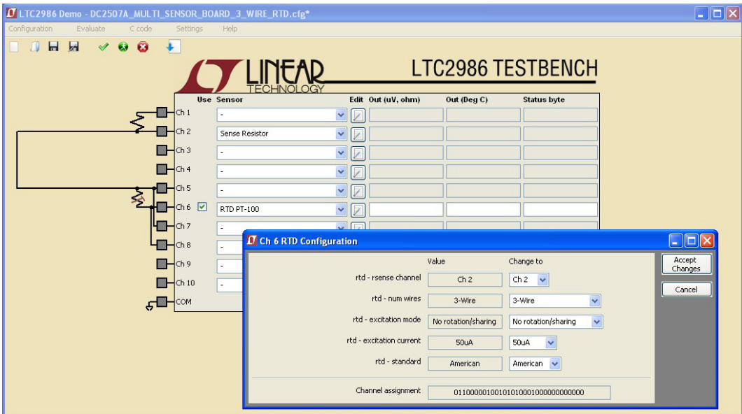
Figure 8. 3-Wire RTD Configuration
