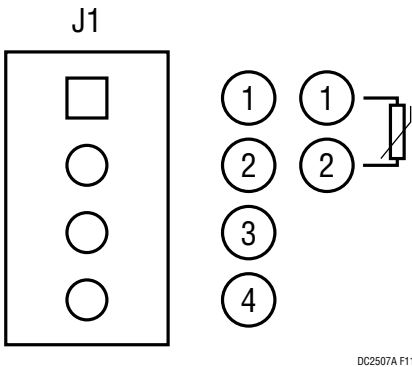
Figure 11. Thermistor Connection
