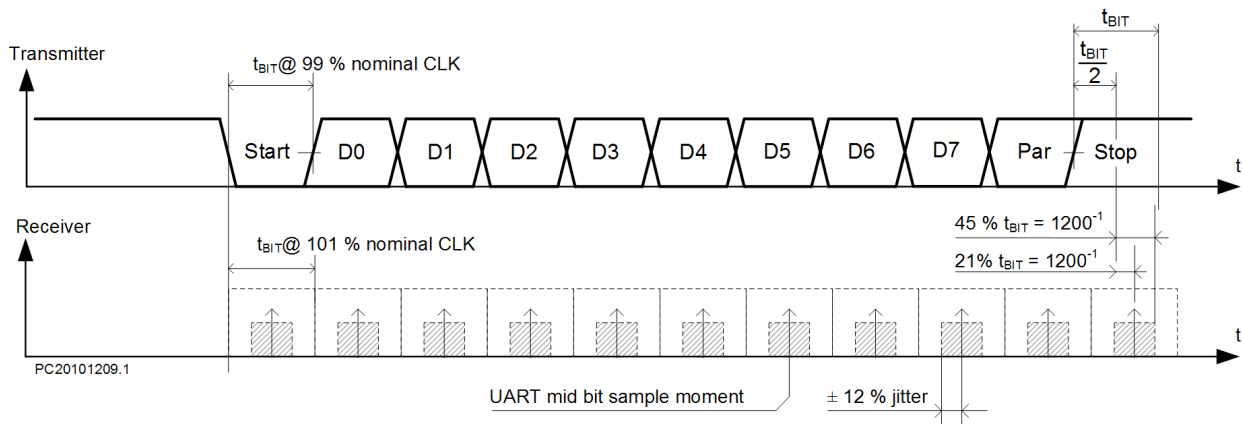
Figure 10. Clock Skew
