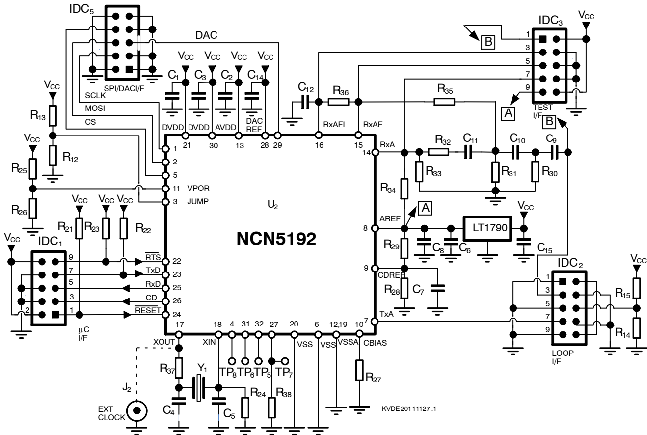
Figure 2. NCN5192NGEVB Schematic
