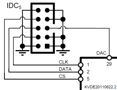
Figure 11. SPI Interface (IDC 5 )
