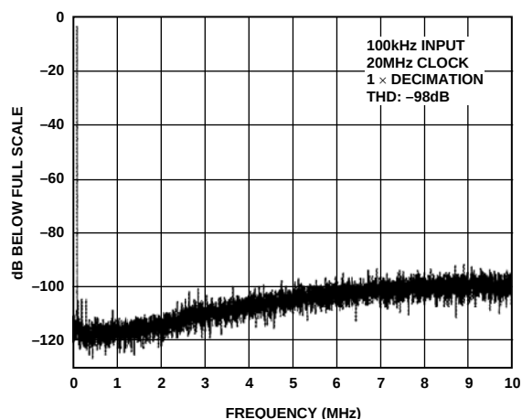
Figure 14. Spectral Plot of the AD9260 at 100 kHz Input, 20 MHz Clock, Undecimated (20 MHz Output Data Rate)
