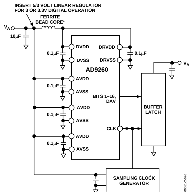
Figure 76. High Frequency Supply Rejection
