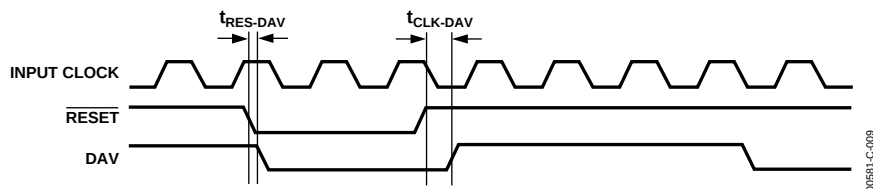
Figure 9. \overline{\text{RESET}} Timing Diagram
