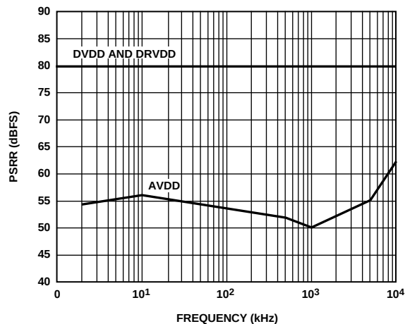
Figure 73. AD9260 PSRR vs. Frequency (8x Mode)
