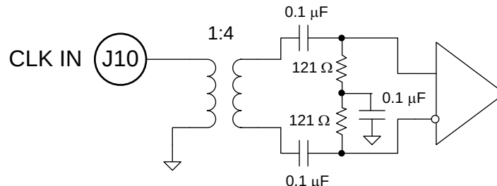
Figure 5. ADS4449 Clock Input Circuit
