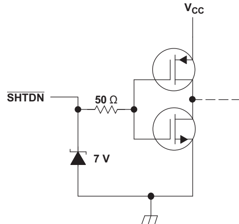
Figure 9. SHTDN Input
