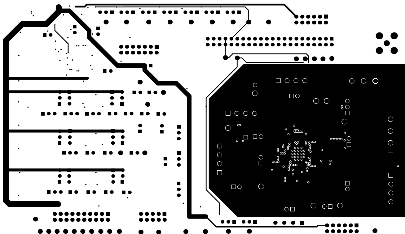
Figure 11. Layer 3 POWER
