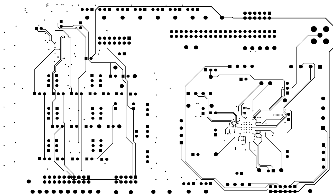
Figure 10. Layer 2 SIGNAL
