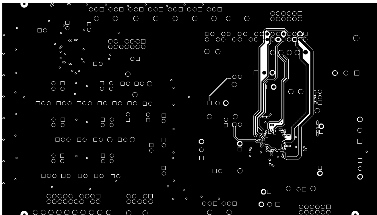
Figure 12. Bottom Layer
