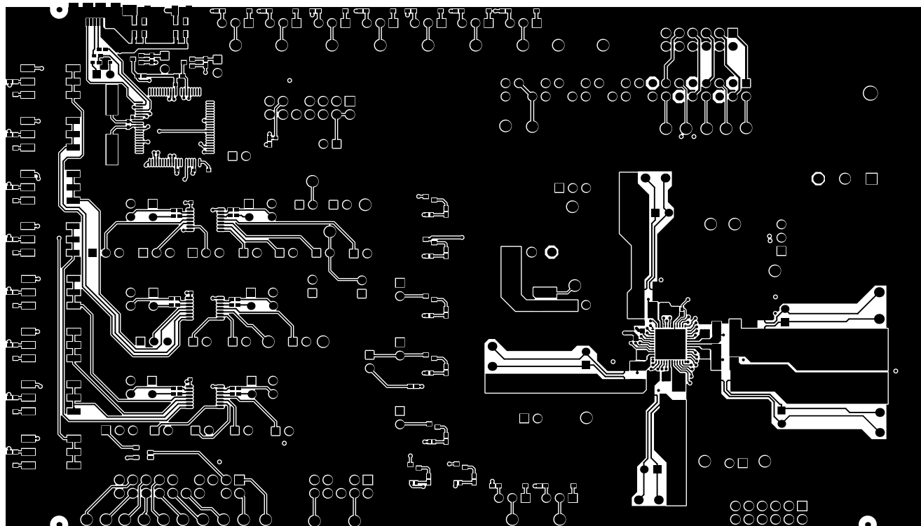
Figure 8. Top Layer
