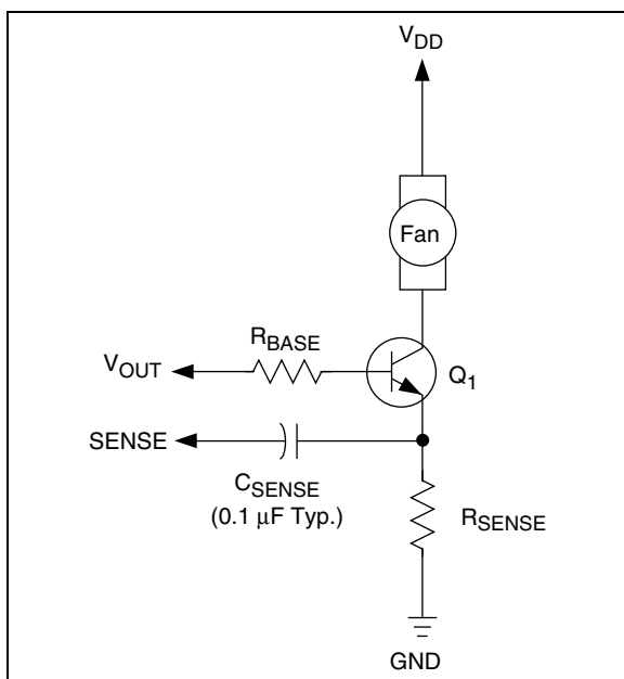
FIGURE 5-4: SENSE Network.
