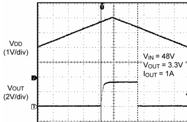
V_{DD} UVLO Thresholds
