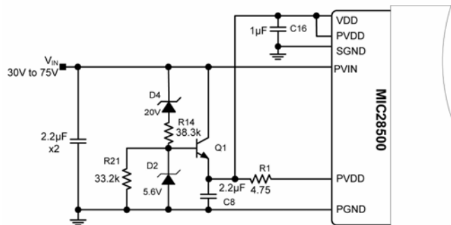
Figure 9B: V_{IN} Limiter On VDD pin
