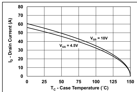
FIGURE 2-10: Maximum Drain Current vs. Temperature 5x6-PDFN (MCP87090T-U/MF).
