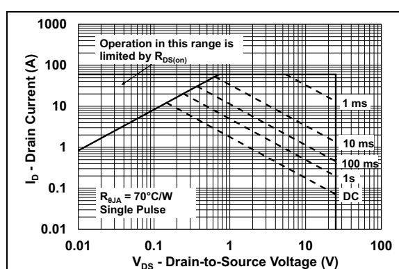
FIGURE 2-12: Maximum Safe Operating Area 3.3x3.3-PDFN (MCP87090T-U/LC).
