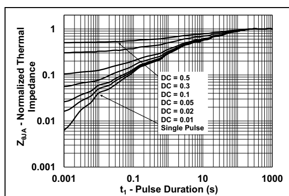
FIGURE 2-11: Transient Thermal Impedance 5x6-PDFN (MCP87090T-U/MF).
