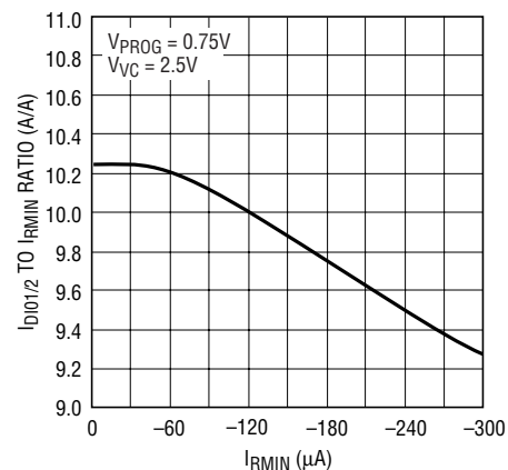
I_{DIO1/2} to I_{RMIN} Ratio vs R_{MIN} Current
