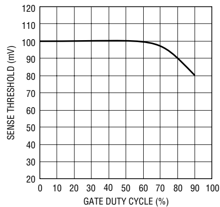
Maximum Sense Threshold vs Gate Drive Duty Cycle
