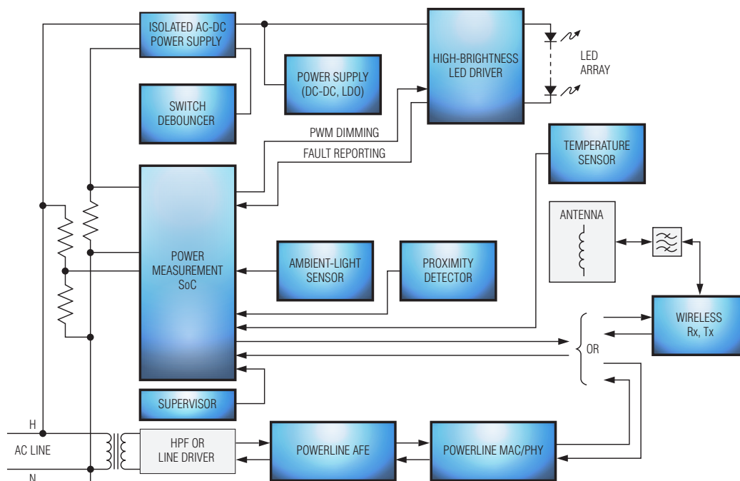
Block diagram of an LED lighting system controlled through PLC or wireless links. View recommended solutions at www.maxim-ic.com/lighting .
