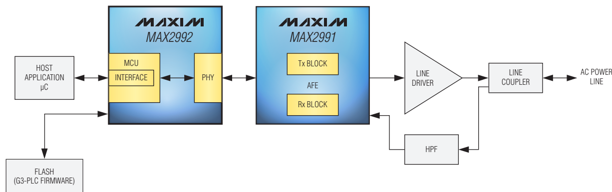
Block diagram of the MAX2991/MAX2992 G3-PLC chipset.
