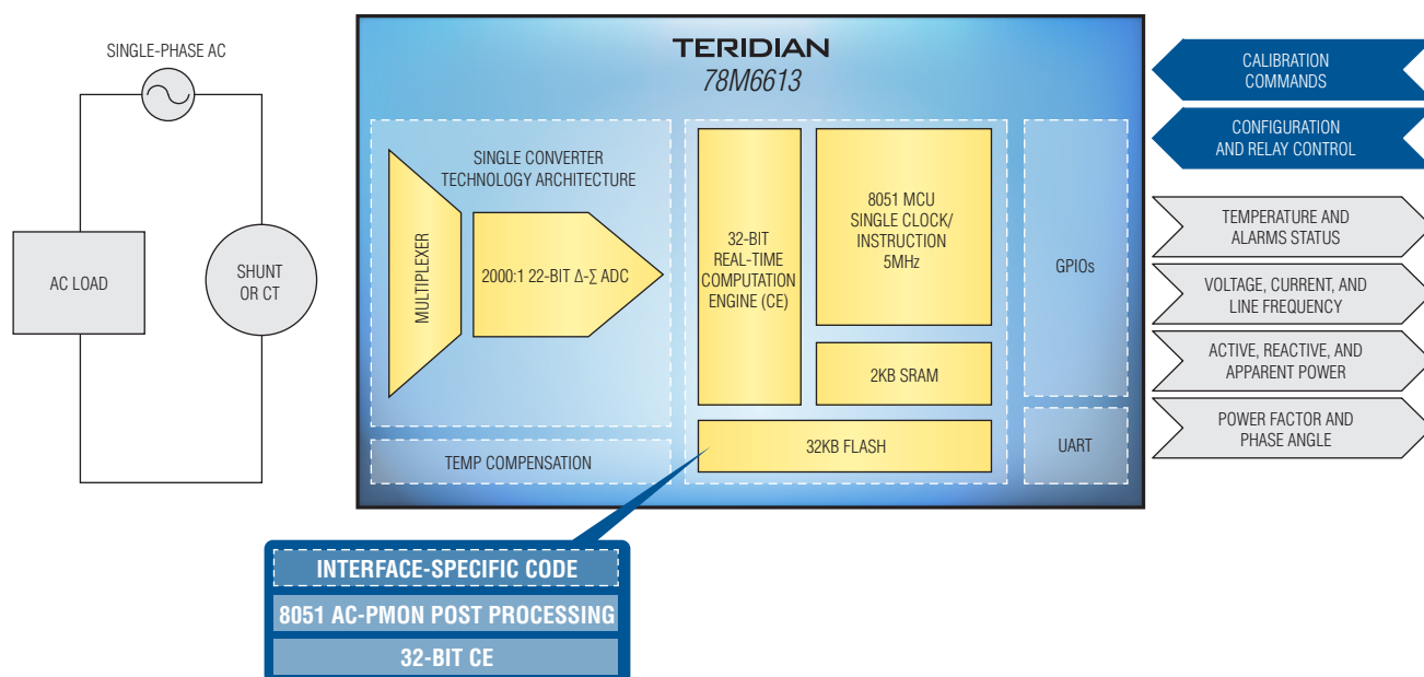
Diagram of the 78M6613 embedded in a single-phase application.
