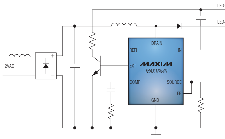
Typical operating circuit for the MAX16840.
