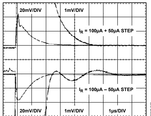
Figure 12. Transient Settling Time
