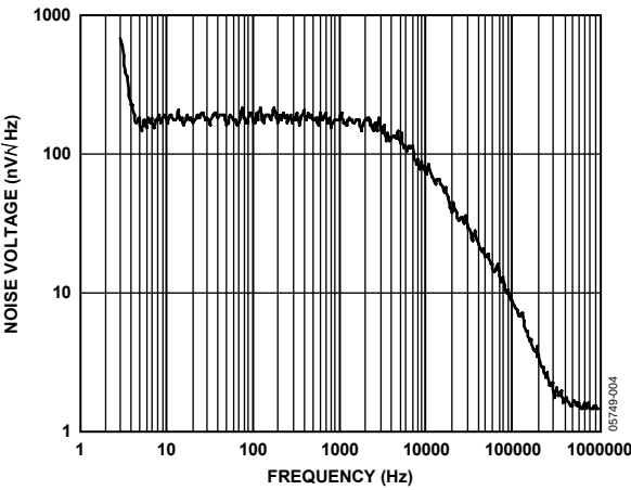
Figure 4. Noise Spectral Density
