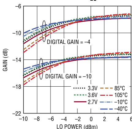
Gain vs LO Power at f_{LO} = 500MHz
