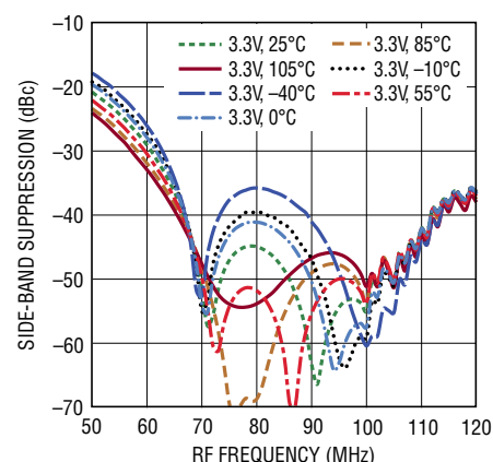
Side-Band Suppression vs RF Frequency for 70MHz LO Match
