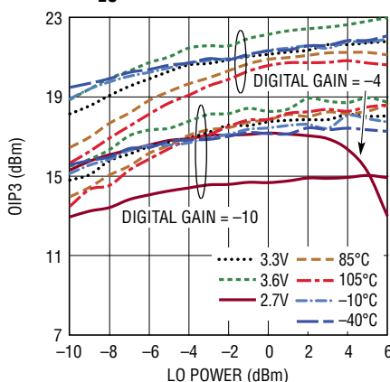
Output IP3 vs LO Power at f_{LO} = 150MHz
