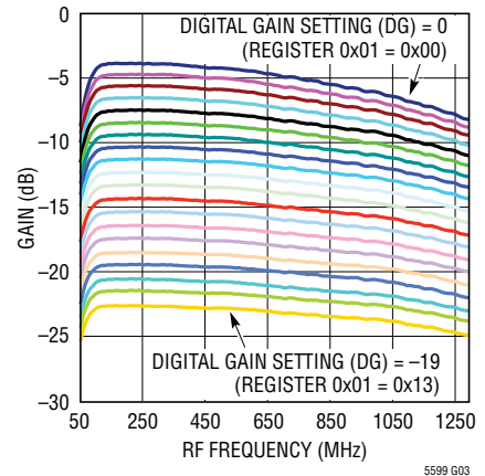
Gain vs RF Frequency and Digital Gain Setting
