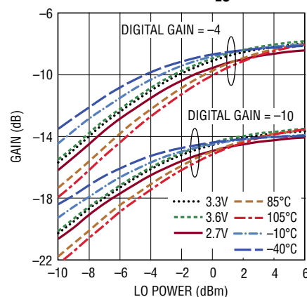
Gain vs LO Power at f_{LO} = 900MHz
