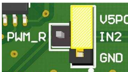
Figure 8. IN2 Connected to V5P0 (Logic High)
