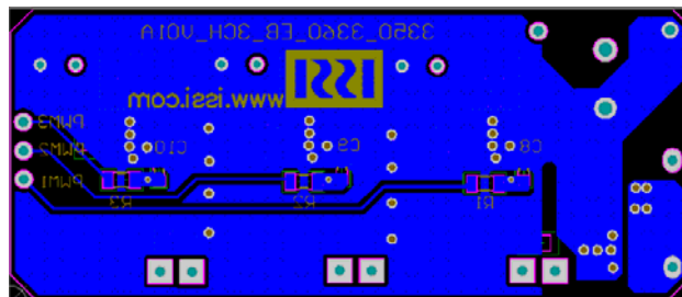
Figure 3 PCB Layout-Bottom Layer
