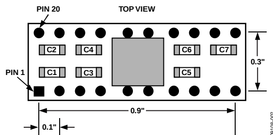
Figure 2. EVAL-ADXRS620 Parts Layout
