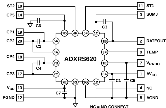
Figure 1. EVAL-ADXRS620 Schematic
