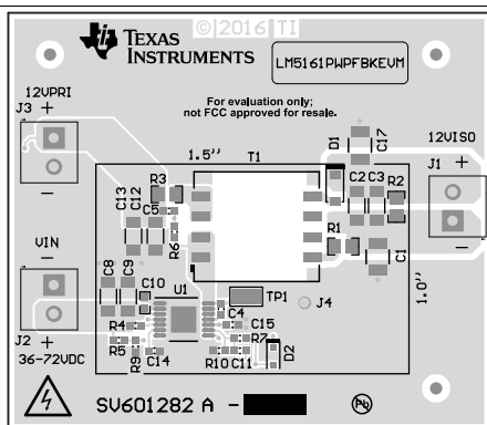
Figure 11. EVM Component View (Top)
