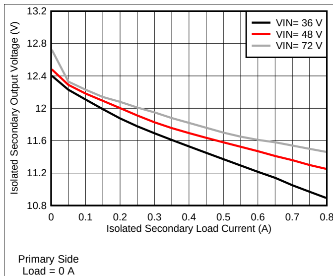
Figure 2. Secondary Side ( V_{OUTISO} ) Load Regulation
