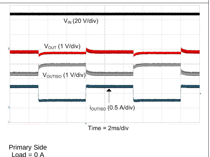
Figure 5. Secondary Isolated Output Load Transient at V_{IN} = 48 V and I_{OUTISO} = 250 mA to 750 mA
