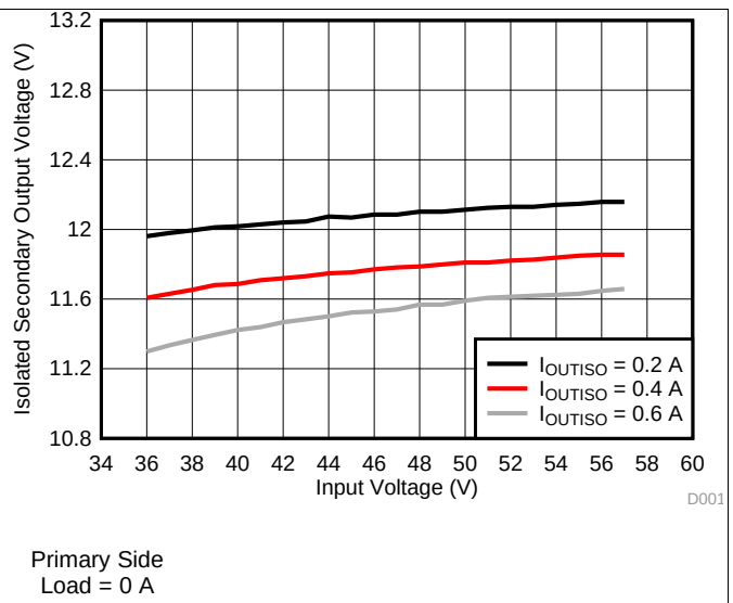
Figure 3. Secondary Side ( V_{OUTISO} ) Line Regulation
