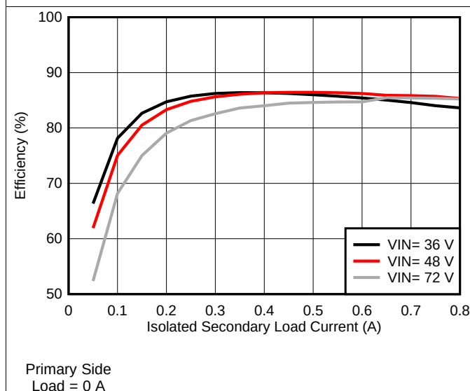
Figure 4. Efficiency vs I_{OUTISO} with Default Board Configuration
