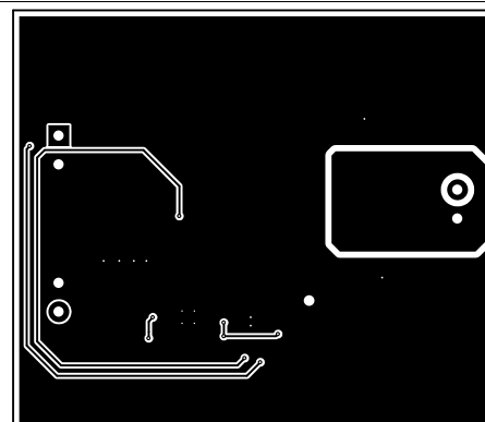
Figure 14. EVM Copper View (Bottom)
