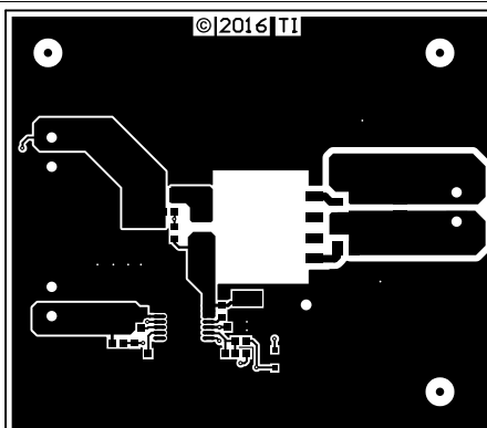
Figure 13. EVM Copper View (Top)
