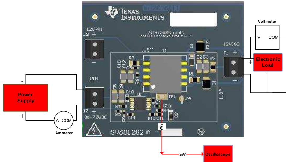
Figure 1. EVM Test Setup
