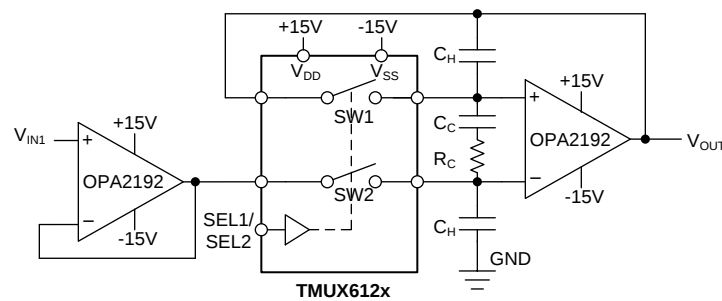
Figure 31. A Sample and Hold Circuit Realized Using the TMUX611x Analog Switch
