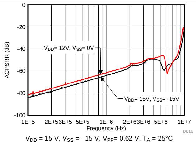
Figure 14. ACPSRR vs Frequency
