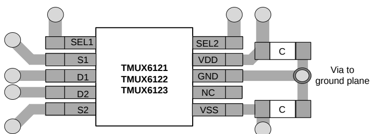
Figure 34. TMUX6121 Layout Example
