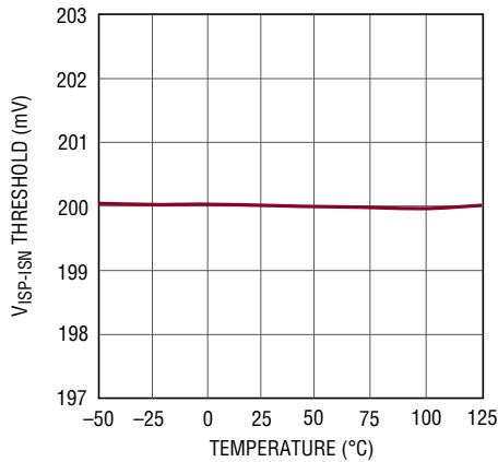
V_{\text{ISP-ISN}} Threshold at \text{CTRL} = 0.7\text{V} vs Temperature
