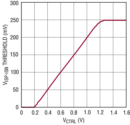
V_{\text{ISP-ISN}} Threshold vs V_{\text{CTRL}}
