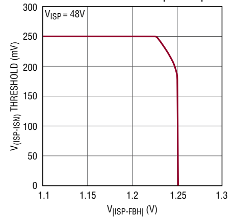
V_{\text{ISP-ISN}} Threshold vs V_{\text{ISP-FBH}}
