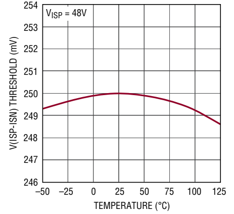
V_{\text{ISP-ISN}} Full-Scale Threshold vs Temperature
