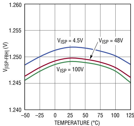
|V_{\text{ISP-FBH}}| Regulation Voltage vs Temperature, V_{\text{ISP}}
