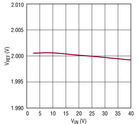
V_{\text{REF}} Voltage vs V_{\text{IN}}
