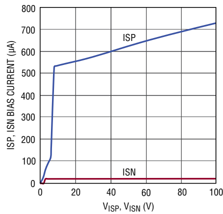
ISP/ISN Input Bias Current vs V_{\text{ISP}} , V_{\text{ISN}}
