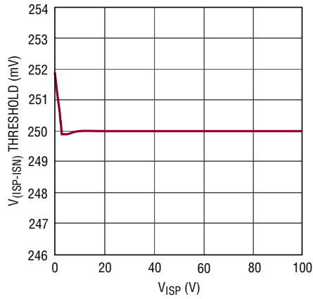
V_{\text{ISP-ISN}} Threshold vs V_{\text{ISP}}
