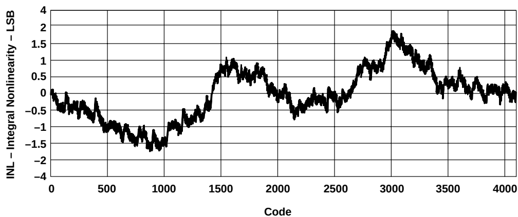
Figure 13. Integral Nonlinearity
