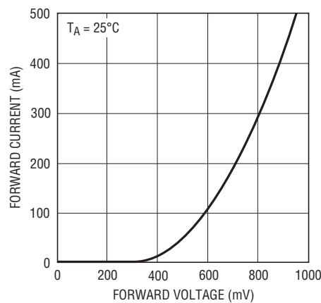
Schottky Forward Voltage Drop
