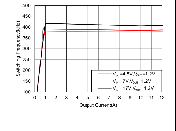
Figure 18. F_{SW} Load Regulation, Mode = DCM, F_{SW} = 400\text{kHz}
