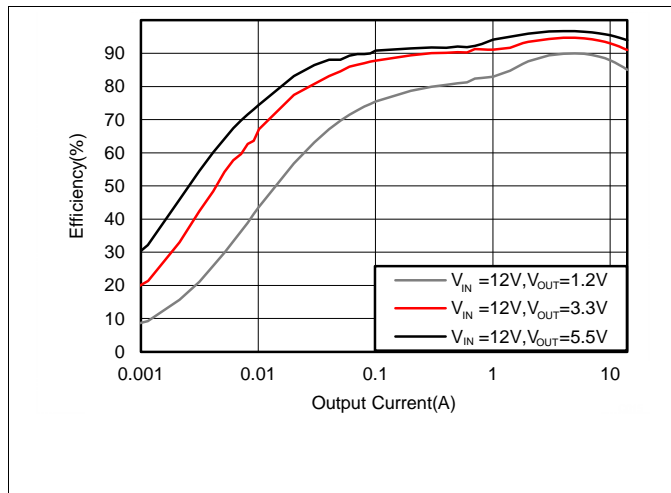
Figure 13. Efficiency, Mode = DCM, F_{SW} = 400\text{kHz}
