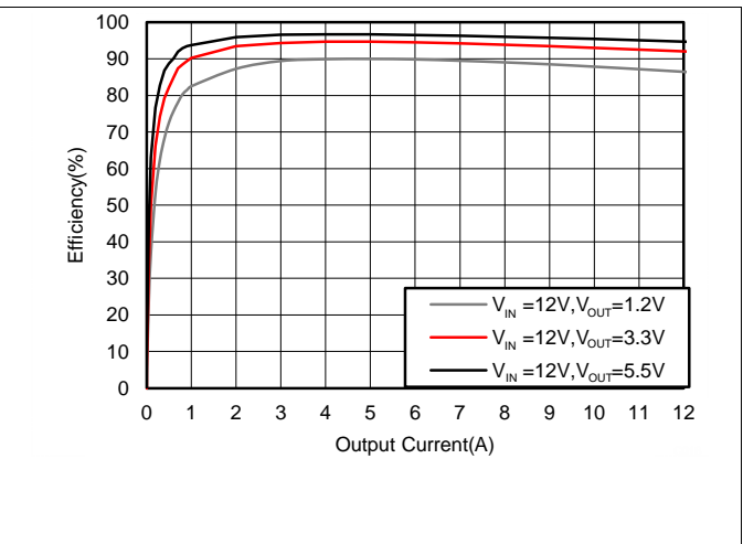
Figure 14. Efficiency, Mode = FCCM, F_{SW} = 400\text{kHz}
