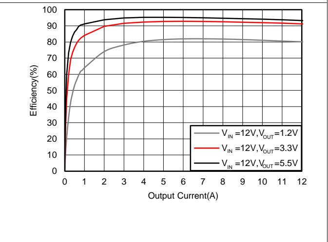
Figure 16. Efficiency, Mode = FCCM, F_{SW} = 1200\text{kHz}
