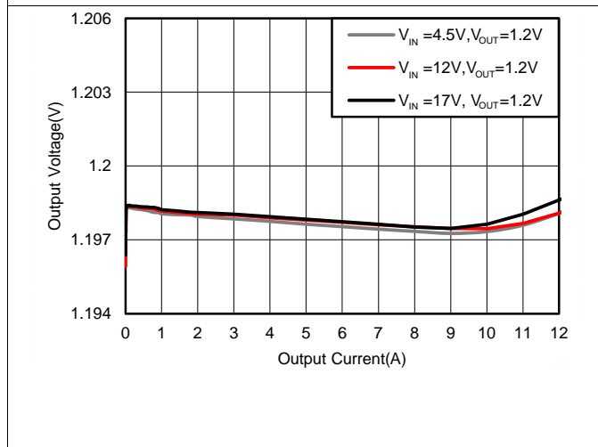
Figure 17. Load Regulation, F_{SW} = 800\text{kHz}
