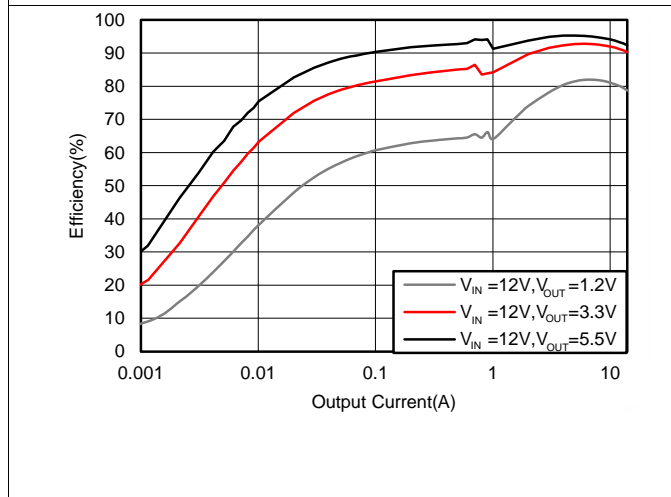
Figure 15. Efficiency, Mode = DCM, F_{SW} = 1200\text{kHz}
