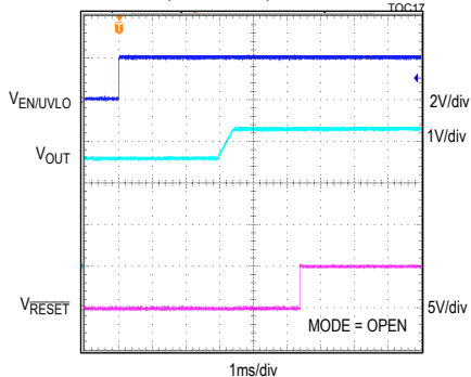
SOFT-START WITH 2.5V PREBIAS, 3.3V OUTPUT, PFM MODE, FIGURE 4B CIRCUIT TOC17
