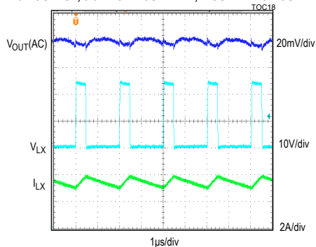
STEADY-STATE SWITCHING WAVEFORMS, 5V OUTPUT, 3.5A LOAD CURRENT, FIGURE 4A CIRCUIT
