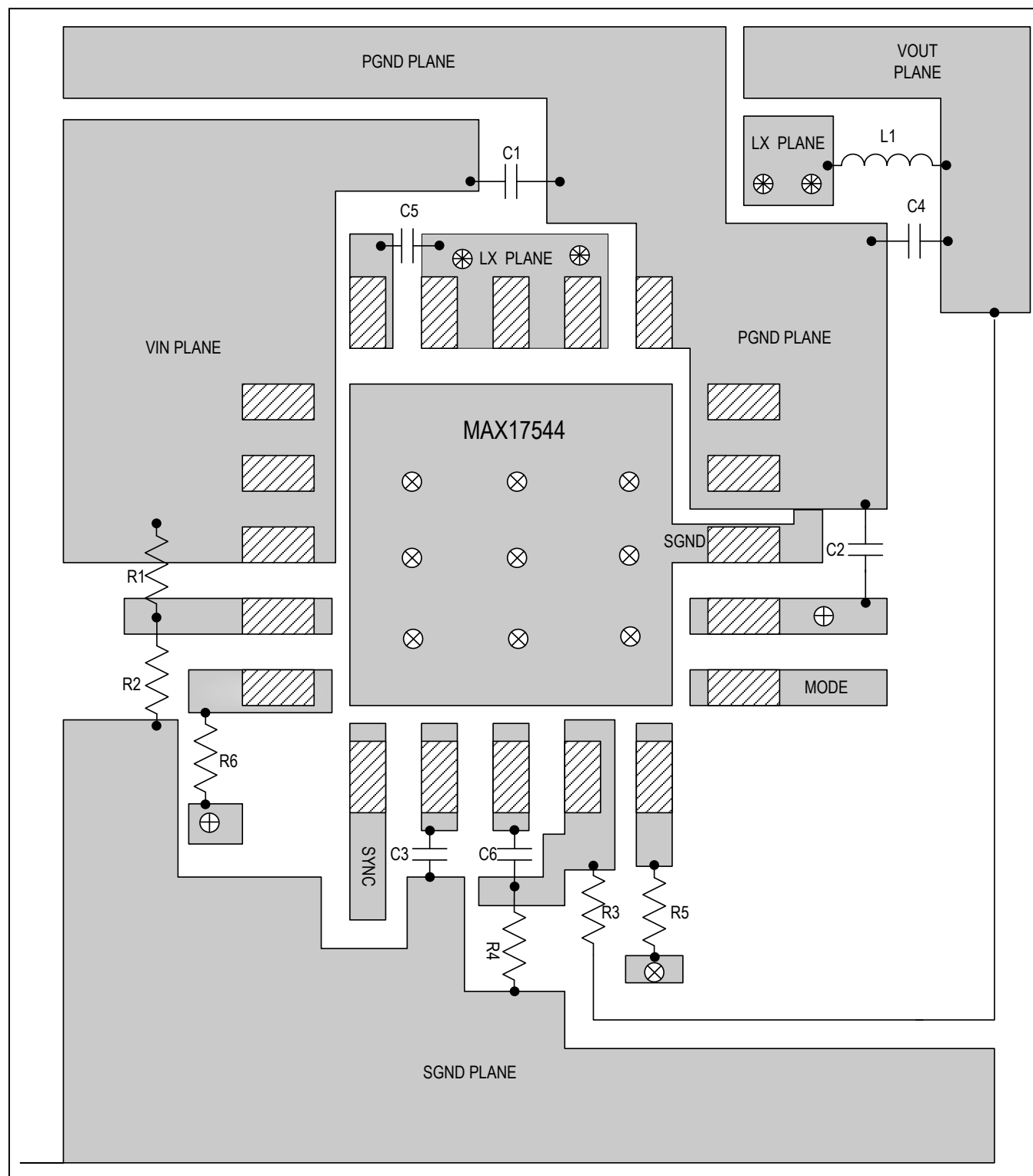
Figure 3b. Layout Guidelines
