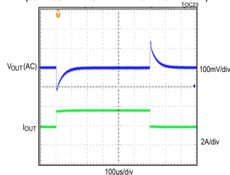
3.3V OUTPUT, PWM MODE, FIGURE 4B CIRCUIT (LOAD CURRENT STEPPED FROM 1.75A TO 3.5A)
