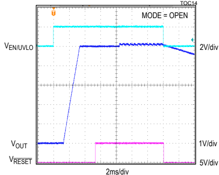
SOFT-START/SHUTDOWN FROM EN/UVLO, 5V OUTPUT, PFM MODE, 5mA LOAD CURRENT, FIGURE 4A CIRCUIT TOC14
