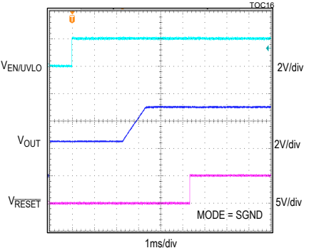
SOFT-START WITH 2.5V PREBIAS, 5V OUTPUT, PWM MODE, FIGURE 4A CIRCUIT TOC16
