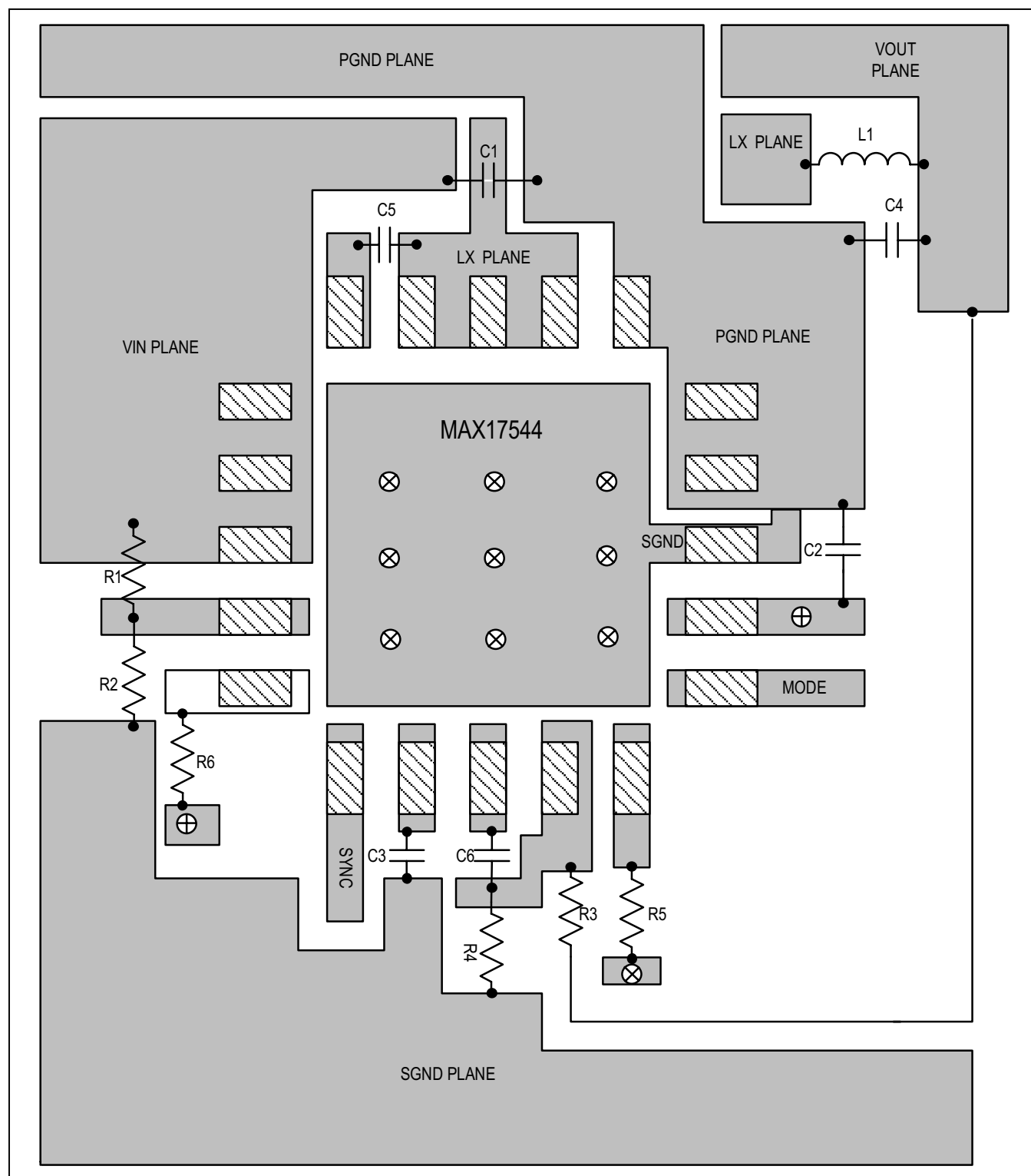
Figure 3a. Layout Guidelines
