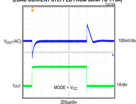
3.3V OUTPUT, DCM MODE, FIGURE 4B CIRCUIT (LOAD CURRENT STEPPED FROM 50mA TO 1.75A)
