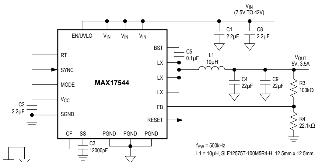
Figure 4a - 5V Output, 500kHz Switching Frequency
