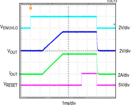
SOFT-START/SHUTDOWN FROM EN/UVLO, 3.3V OUTPUT, 3.5A LOAD CURRENT, FIGURE 4B CIRCUIT TOC13
