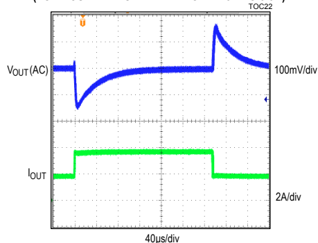
5V OUTPUT, PWM MODE, FIGURE 4A CIRCUIT (LOAD CURRENT STEPPED FROM 1.75A TO 3.5A)
