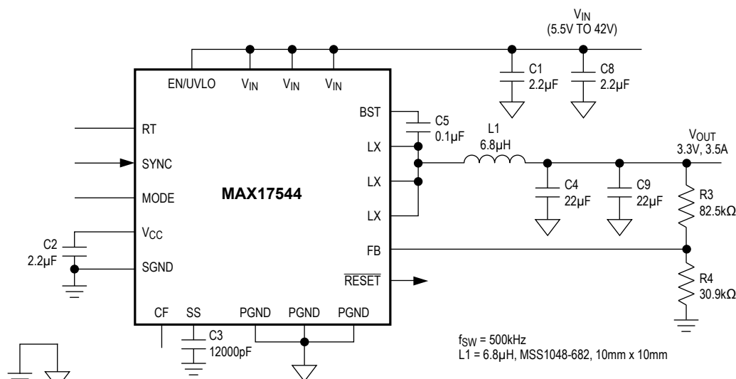
Figure 4b - 3.3V Output, 500kHz Switching Frequency
