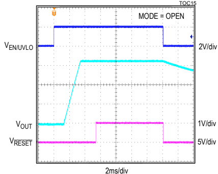
SOFT-START/SHUTDOWN FROM EN/UVLO, 3.3V OUTPUT, PFM MODE, 5mA LOAD CURRENT, FIGURE 4B CIRCUIT TOC15
