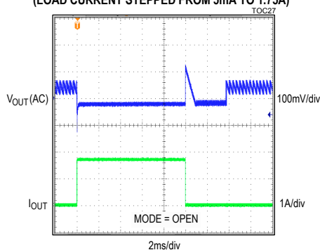
3.3V OUTPUT, PFM MODE, FIGURE 4B CIRCUIT (LOAD CURRENT STEPPED FROM 5mA TO 1.75A)
