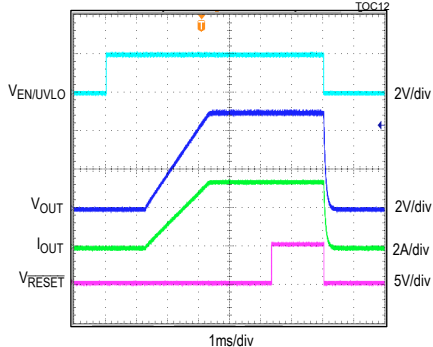
SOFT-START/SHUTDOWN FROM EN/UVLO, 5V OUTPUT, 3.5A LOAD CURRENT, FIGURE 4A CIRCUIT TOC12
