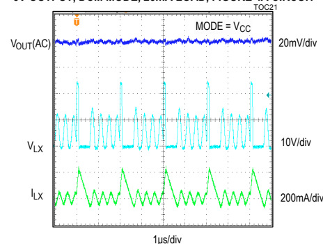
STEADY-STATE SWITCHING WAVEFORMS, 5V OUTPUT, DCM MODE, 25mA LOAD, FIGURE 4A CIRCUIT
