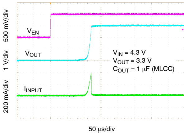
Figure 32. Enable Turn-on Response – C_{OUT} = 1\text{ }\mu\text{F} , I_{OUT} = 10\text{ mA}
