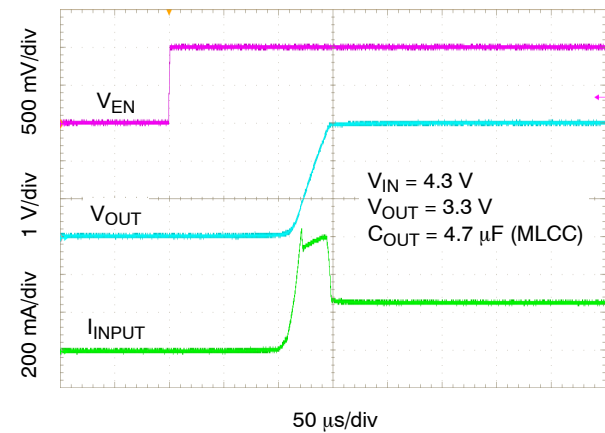
Figure 35. Enable Turn-on Response – C_{OUT} = 4.7\text{ }\mu\text{F} , I_{OUT} = 250\text{ mA}
