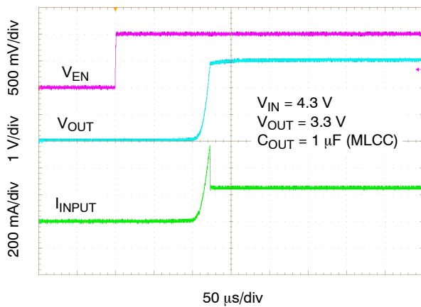
Figure 34. Enable Turn-on Response – C_{OUT} = 1\text{ }\mu\text{F} , I_{OUT} = 250\text{ mA}
