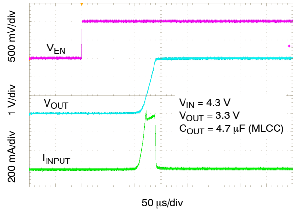
Figure 33. Enable Turn-on Response – C_{OUT} = 4.7\text{ }\mu\text{F} , I_{OUT} = 10\text{ mA}
